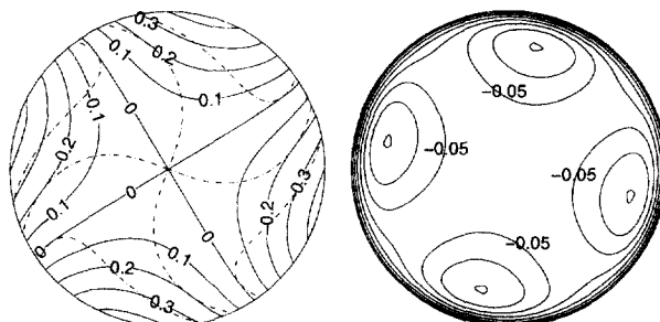
a) – A_z = 0.1k and k = [-4, 4] . - - - A_z = 0.1k and k = [-1, 1] . b) \psi = -0.01k and k = [0, 7] .
