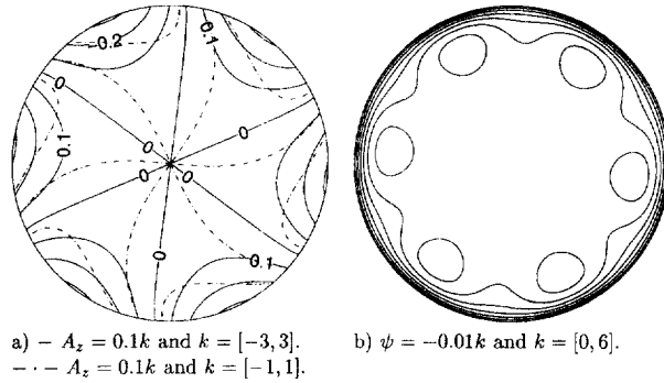
Fig. 12. - Same legend as figure 11 for p = 3 , Ha = 30 and R_\omega = 7 .
