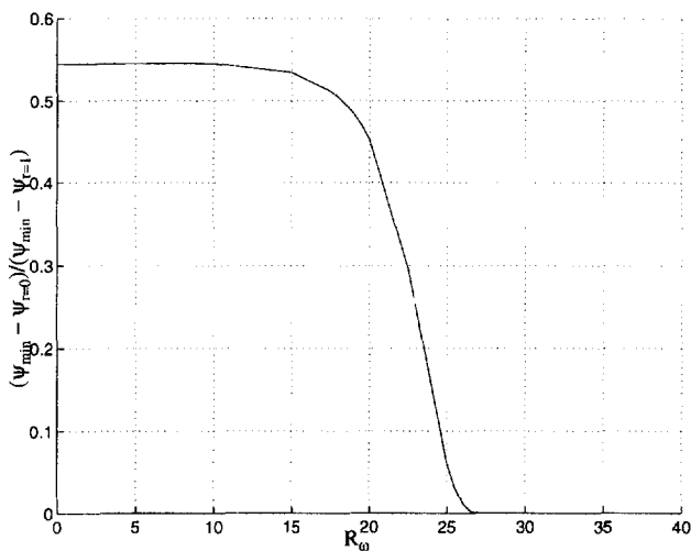
Fig. 10. – Ratio between the recirculating flow rate of one eddy to the total flow rate versus R_\omega for Ha = 30 .
