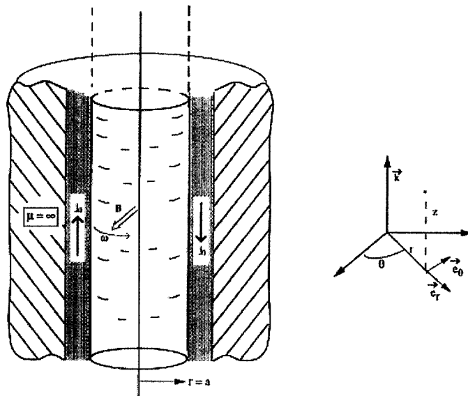
Fig. 2. – Coordinate system.
